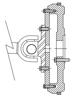
TYPICAL ADAPTER DISK MOUNTING OF CDS50 SERIES DRIVE SHAFTS
